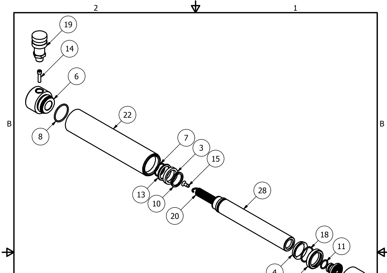
RC-10-SA-8 Parts List
