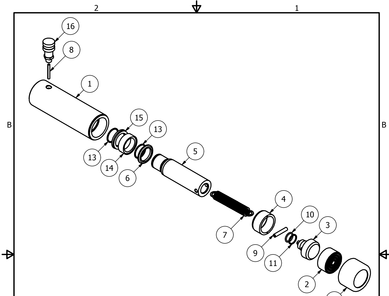
RC-20-SA-6A Parts List
